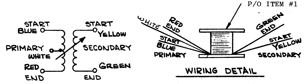
SCHEMATIC DIAGRAM
